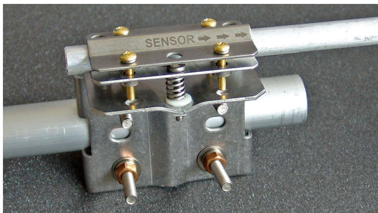
FIGURE 4-2. Attaching the CNR4 onto the mounting rod (pn 26120) using vertical pole or horizontal crossarm
