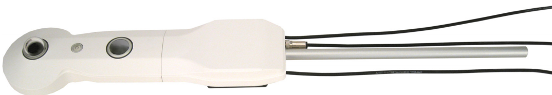
FIGURE 6-2. The CNR4 net radiometer with CNF 4 heater/ventilator unit, top view
