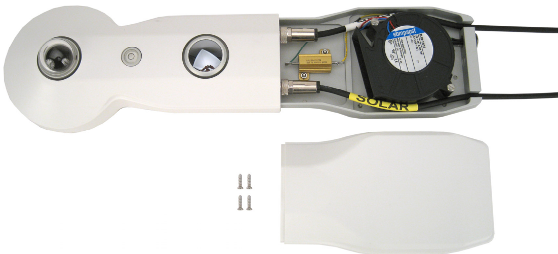
FIGURE B-4. CNF4 solar shield and four flat-head screws
